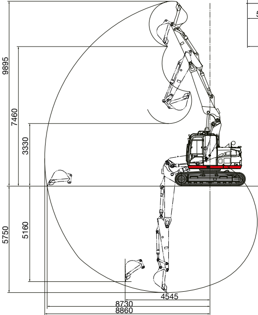
2-piece Boom
